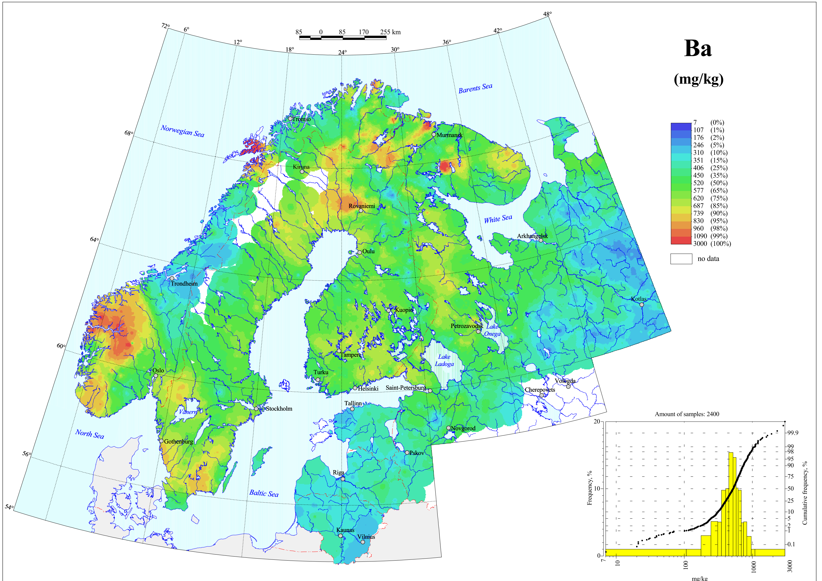
Barium in C-horizon, Grain Size <2 mm, Total Content
